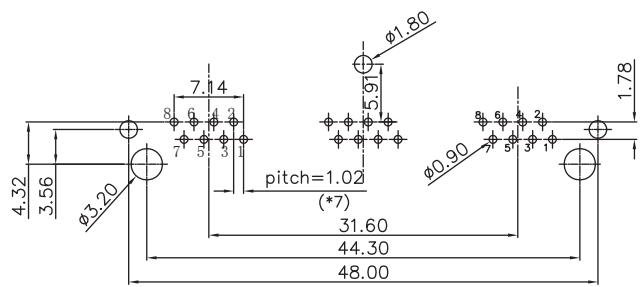
PC Board Layout(t=1.60) Component Side Shown TOLERANCE ±0.08 UNLESS OTHERWISE SPECIFIED
