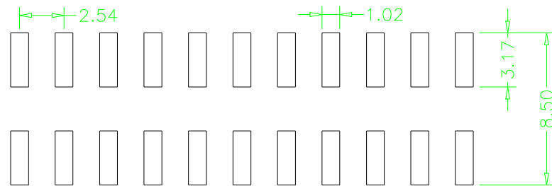
PCB LAYOUT
