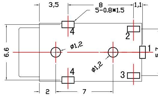
P. C. B TERMINAL POSITION
