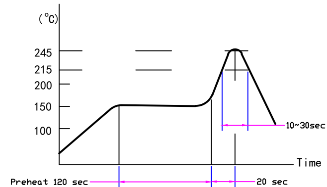
REFLOW SOLDERING CONDITIONS
